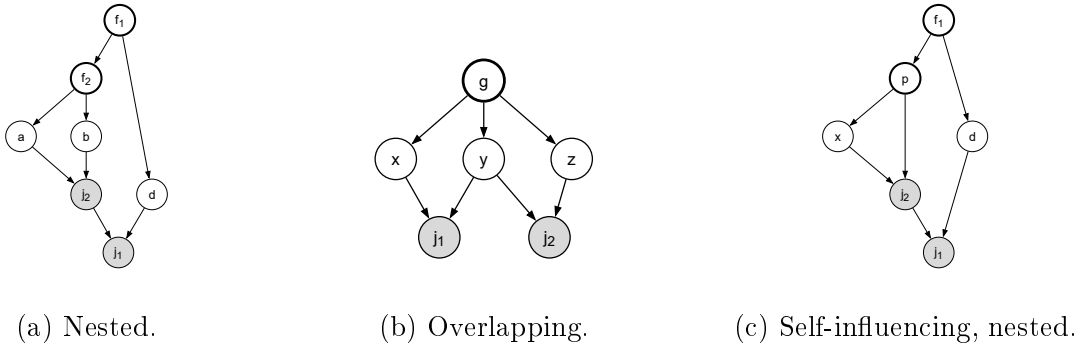
Figure 2: Non-induced diamonds. In (b) two diamonds overlap through the shared fork g , and in (c) parent p is itself the fork of the inner pattern.
